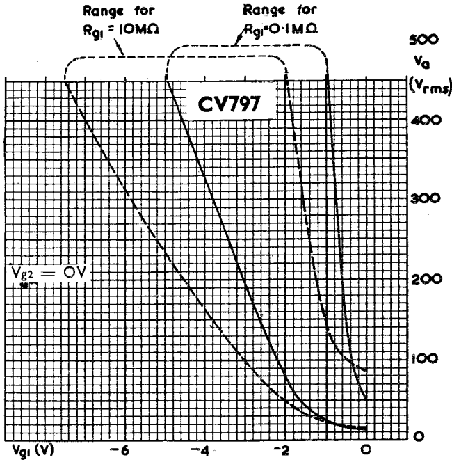
OPERATING RANGE OF CRITICAL GRID VOLTAGE
