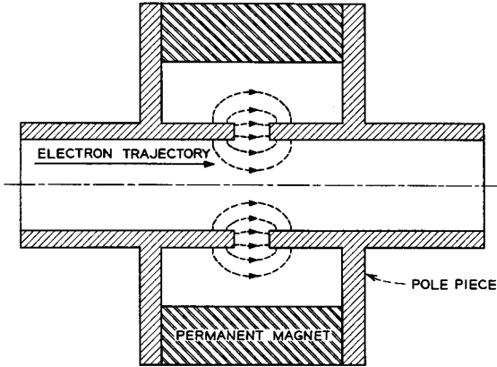
FIG. 3.2-1 A magnetic electron lens.
