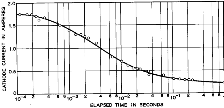
FIG. 2.3-3 The decay of the saturation emission current density drawn from a particular diode when a step-function voltage is applied to the anode. The abscissa indicates time elapsed after application of voltage to the anode. (From L. S. Nergaard, RCA Rev. 13, 464, December 1952)
