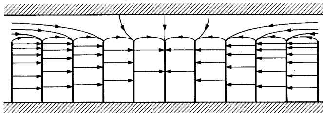
FIG. 8.7-5 Electric field lines in the slow-wave structure of Figure 8.7-4 for \beta_0 L = \pi/10 .
