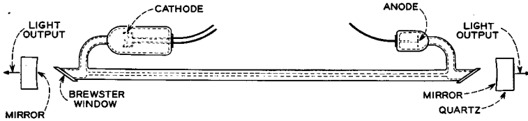
Fig. 17.3-1 The construction of a helium-neon laser.
