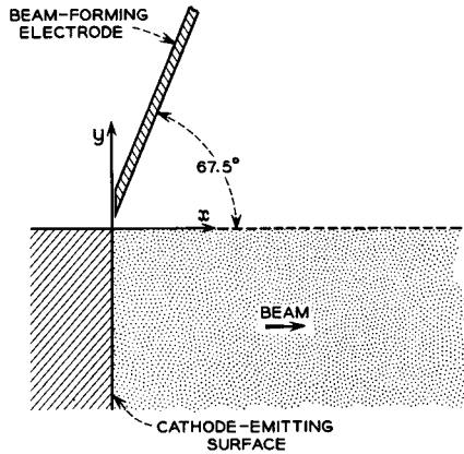
FIG. 4.5-3 An expanded view of the edge of the beam in the region of the cathode.
