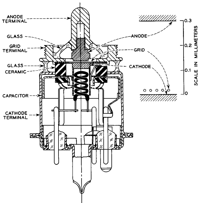
FIG. 7.4-2 The construction of the Western Electric 416B triode. The overall height of the tube is 4.8 cm.
