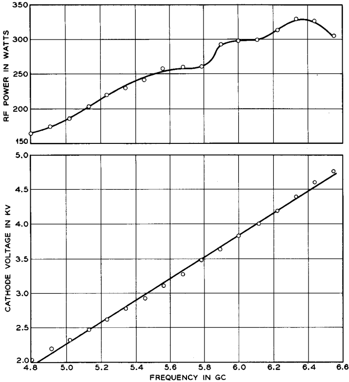
FIG. 12.3-6 Tuning curves for the L-3726. These data correspond to fixed values of sole voltage V_{S_0} and cathode current of 2450 volts and 300 ma, respectively. (Courtesy of Litton Industries, Electron Tube Division)
