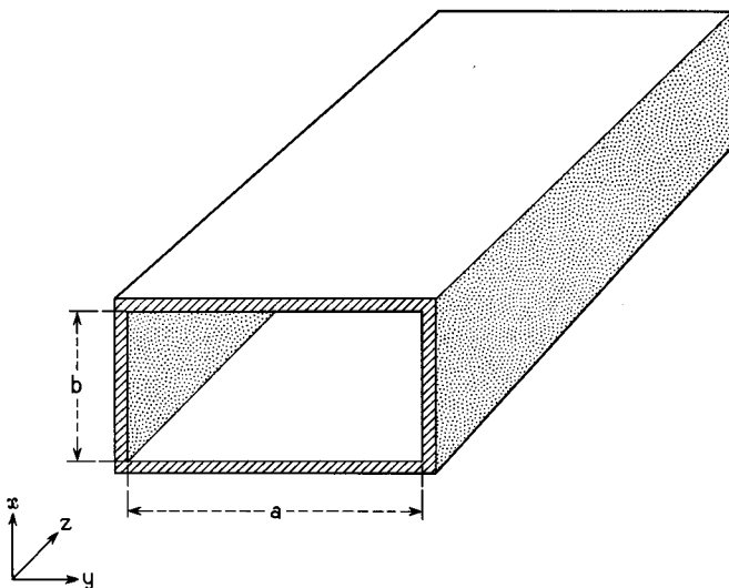
FIG. 8.5-1 Rectangular waveguide.
