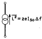
FIG. 13.1-8 Equivalent circuit for the noise from a temperature-limited diode at low frequencies.
