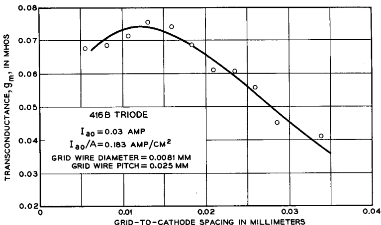
FIG. 5.2-8 Transconductance vs. grid-to-cathode spacing for the 416B triode described in Chapter 7.
