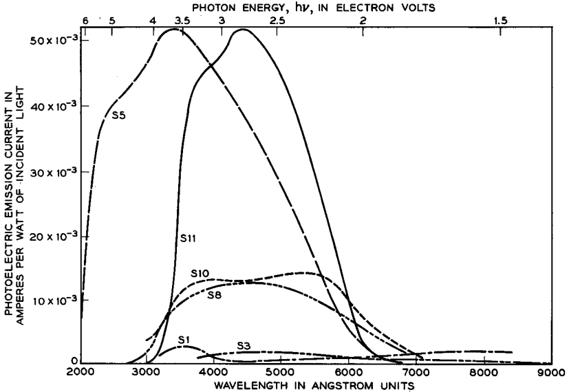
FIG. 2.6-2 Photoelectric emission current from several frequently used compound surfaces as a function of wavelength of the incident light. The curves are for equal values of incident radiant flux at all wavelengths. (Courtesy Allen B. DuMont Laboratories, Inc., Clifton, N.J.)
