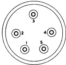
American Medium 5-pin USM5
