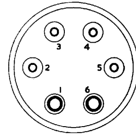
American Medium 6-pin USM6
