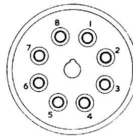
International Octal I.O.
