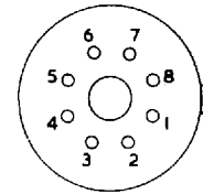
8-pin Glass B8A
