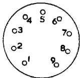
Noval B9A
