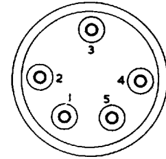
American Small 5-pin USS5
