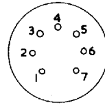
Button Miniature 7-pin Glass B7G
