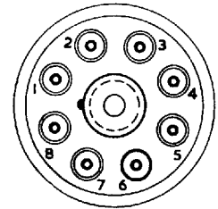
Loctal B8G
