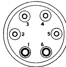
American Small 6-pin USS6
