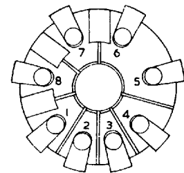
Side Contact SC8
