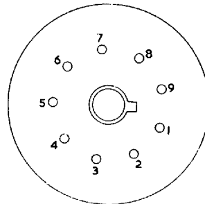
9-pin Glass B9G
