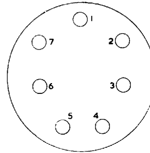
British 7-pin B7
