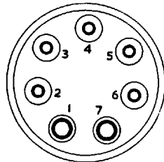
American Small 7-pin USS7
