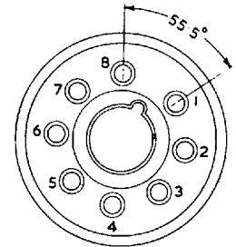
British Octal Mazda Octal M.O.
