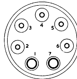
American Medium 7-pin USM7
