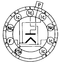
BOTTOM VIEW MINIATURE BUTTON 9 PIN BASE
