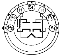
BOTTOM VIEW SUBMINIATURE - 8 FLEXIBLE LEADS
