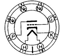
BOTTOM VIEW LOCKING-IN B PIN BASE
