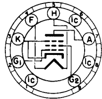
BOTTOM VIEW SMALL BUTTON 9 PIN BASE 9CV
