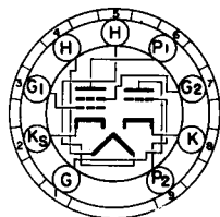
BOTTOM VIEW MINIATURE 9 PIN BASE
