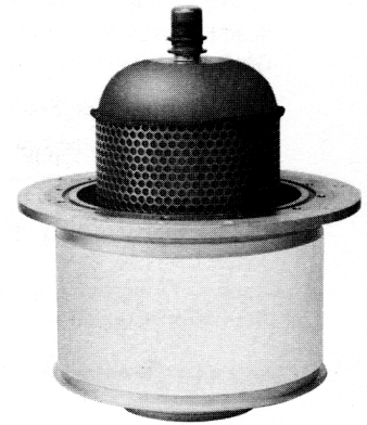
Shown with boiler removed.
